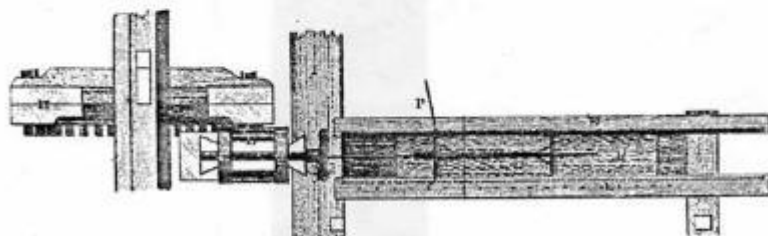
FIGURE 229—(Above) Machinery for boring gun-barrels, with the outside of a barrel being ground on a stone at the rear; (below) plan view of one boring-bench. The rectangular boring-bit of tempered steel, 10 in long, is welded to an iron rod 3\frac{1}{2} ft long (n) rotated by water-power through the wooden gearing. Upon the bench (h) slides a carriage holding the barrel, which is forced on the bit by a lever (v) acting upon the fixed pins. Twenty-two bits, successively larger, are used to enlarge the bore of the barrel from \frac{3}{8} in to \frac{7}{8} in. The trough (v) holds water for cooling.
